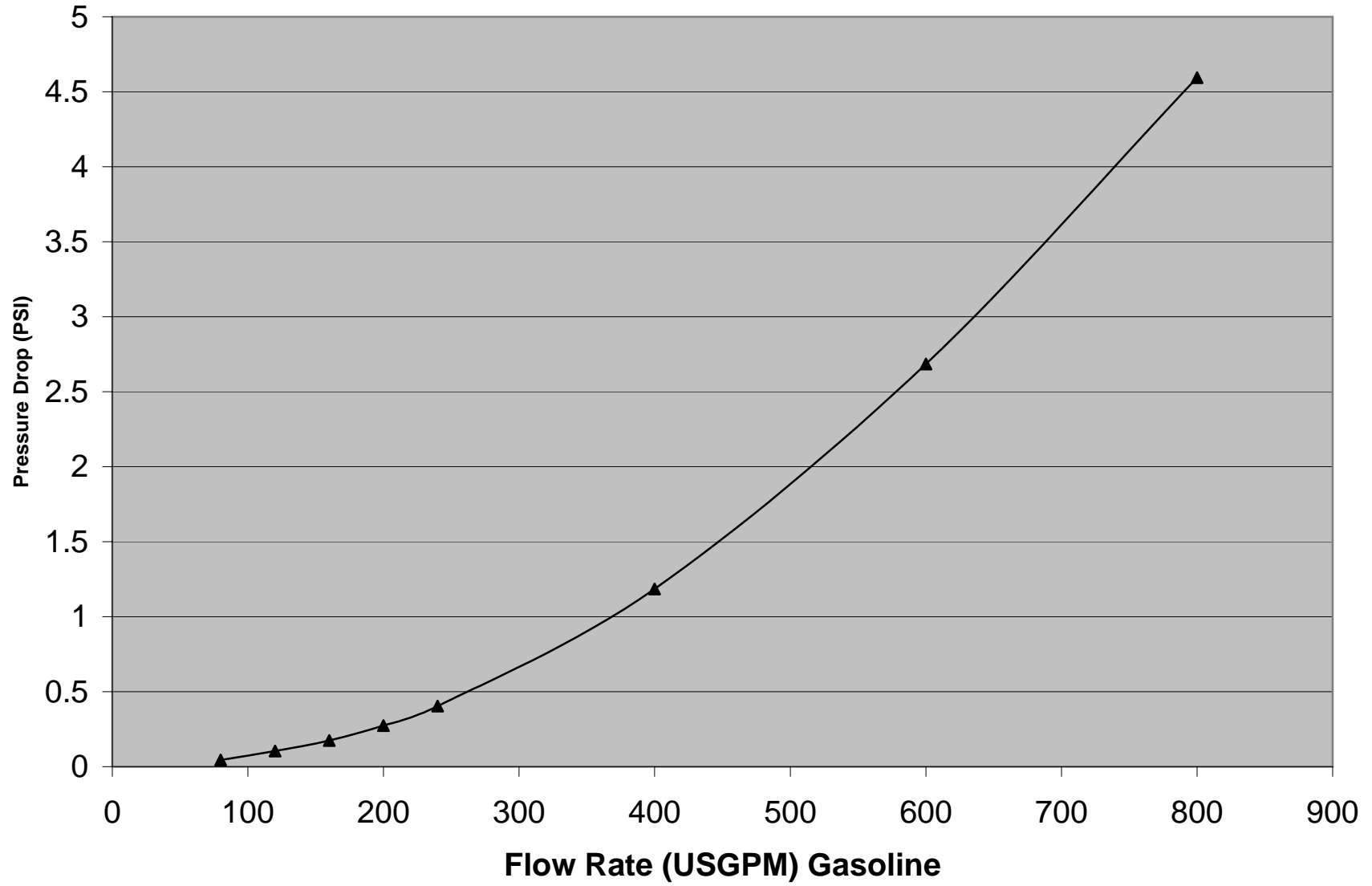
5204 API - Pressure Drop Vs Unloading Flow Rate
