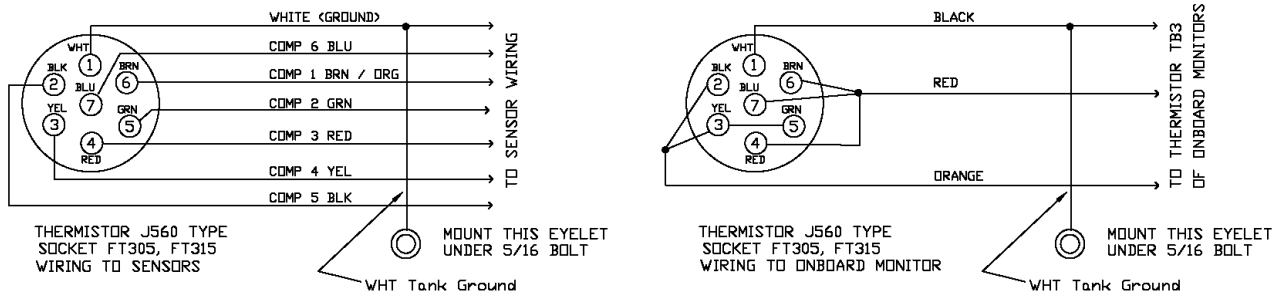
VIEWED FROM WIRE CONNECTION SIDE
