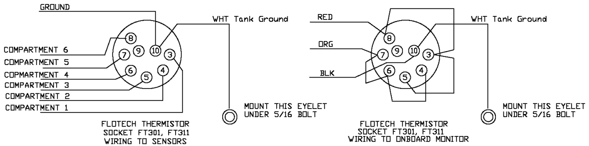
VIEWED FROM WIRE CONNECTION SIDE
