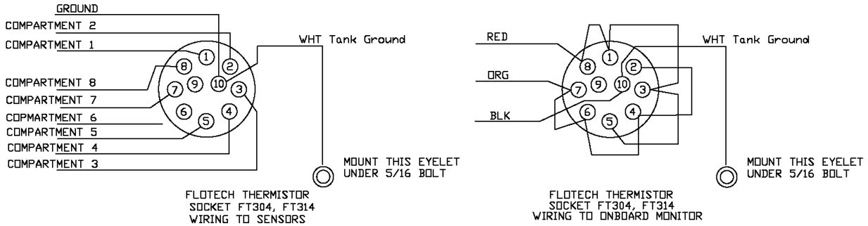
VIEWED FROM WIRE CONNECTION SIDE
