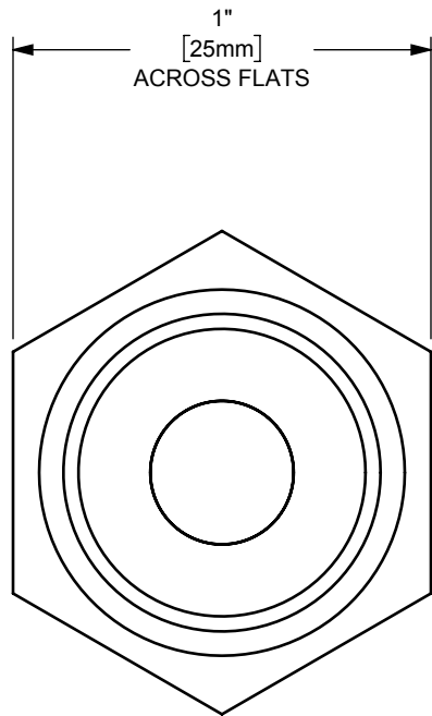
1/2" FEMALE NPSM WITH RUBBER WASHER
